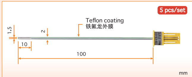
Type E model : STN-41E-010 Type K model : STN-41K-010
