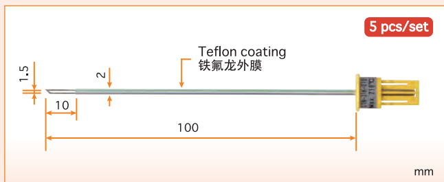
Type E model : STN-31E-010 Type K model : STN-31K-010
