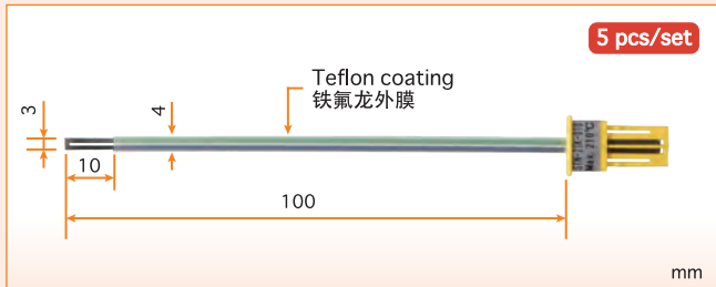
Type E model : STN-21E-010 Type K model : STN-21K-010
