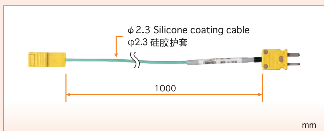
Type E model : STN-E-TS1-ANP Type K model : STN-K-TS1-ANP
